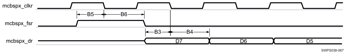
Figure 6-41. McBSP Falling Edge Receive Timing in Slave Mode
