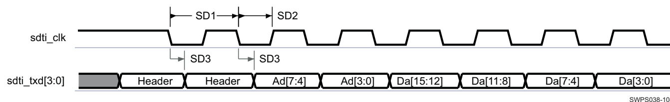
Figure 6-81. SDTI—Single-Edge Mode
