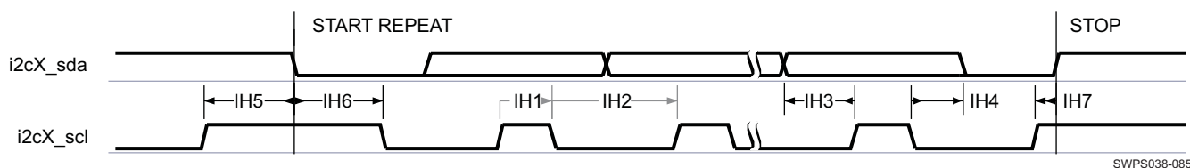
Figure 6-54. I²C—High-Speed Mode
